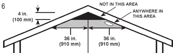
FIGURE 6: RECOMMENDED SMOKE ALARM LOCATION IN ROOMS WITH SLOPED, GABLED, OR PEAKED CEILINGS.
