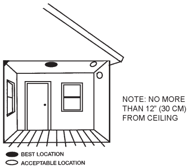
FIGURE 5: RECOMMENDED SMOKE ALARM MOUNTING LOCATIONS.
