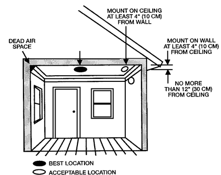
FIGURE 6: RECOMMENDED HEAT ALARM MOUNTING LOCATIONS
